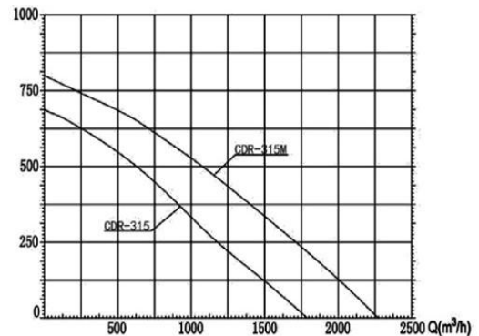
CDR2E-315; CDR2E-315M
