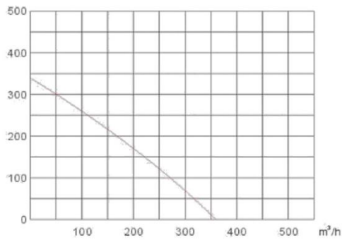
CDR2E-100
